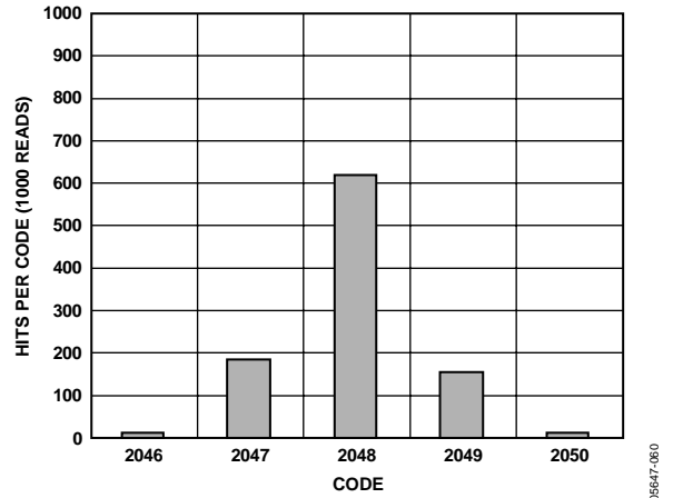
Figure 25. ADC Noise, Current Channel, Midcode Input, 1000 Reads
