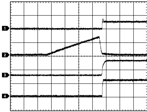
Figure 41. Inrush Current Control into 220 \mu F Load (CH1 = I_{LOAD} , CH2 = V_{TIMER} , CH3 = V_{GATE} , CH4 = V_{OUT} )
