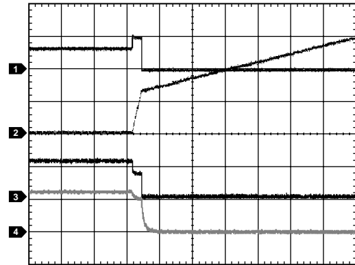
Figure 44. Overcurrent Condition During Operation (ADM1175-1 Model) (CH1 = I_{LOAD} , CH2 = V_{TIMER} , CH3 = V_{GATE} , CH4 = V_{OUT} )
