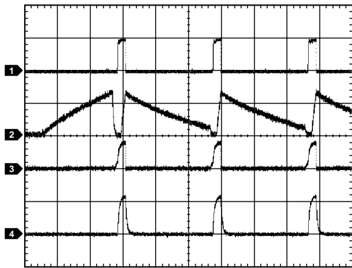
Figure 42. Overcurrent Condition at Startup (ADM1175-1 Model) (CH1 = I_{LOAD} , CH2 = V_{TIMER} , CH3 = V_{GATE} , CH4 = V_{OUT} )
