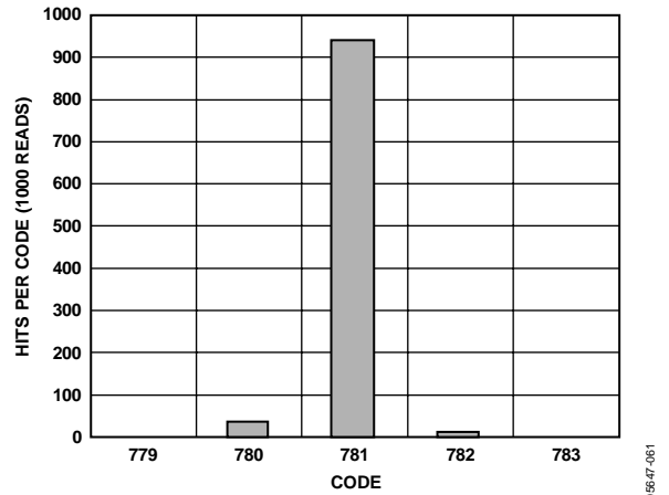
Figure 26. ADC Noise, 14:1 Voltage Channel, 5 V Input, 1000 Reads
